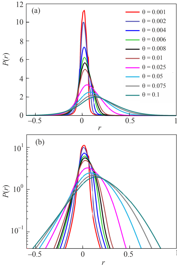
Fig. 2. (Color online) Probability-density function P(r) of the Lyapunov observable r for the SRN case with g = 1 . Panel (a) shows the PDF on linear scales, while panel (b) presents the same data with the y axis plotted on a \log_{10} scale. The colors corresponding to different values of \theta in (a) and (b) are shown in the legend of panel (a). The unitary map Eq. (1) is iterated 10^9 times, yielding 10^9 values for r(t) that were all used to calculate P(r) . The number of unit cells in the system is N = 100 .
