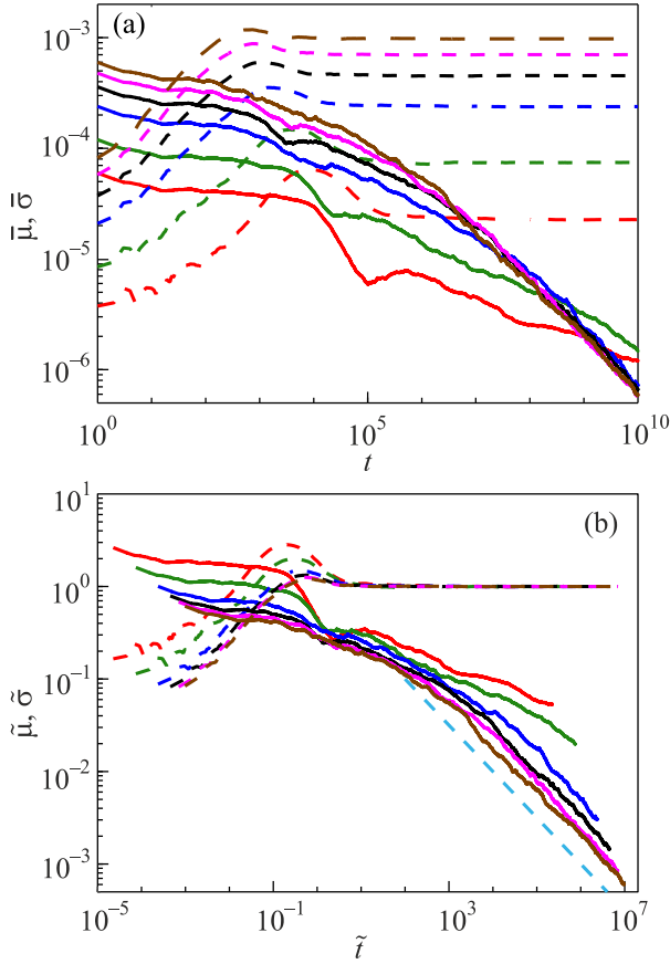
Fig. 7. (Color online) The unscaled (a) and scaled (b) average values of the mean and standard deviation of \Lambda(t) on a \log_{10} scale for the LRN case with \theta = 0.33\pi for different values of g (see main text for more information). The colors red, green, blue, black, magenta, and brown correspond to g = 0.001, 0.002, 0.004, 0.006, 0.008 , respectively. Averaging is performed over 100 trajectories at each time step. In (b), the cyan dashed line indicates the temporal decay \sigma \sim t^{-1/2} . The time evolution is plotted on a \log_{10} scale, extending up to 10^{10} . The number of unit cells is N = 50 .
