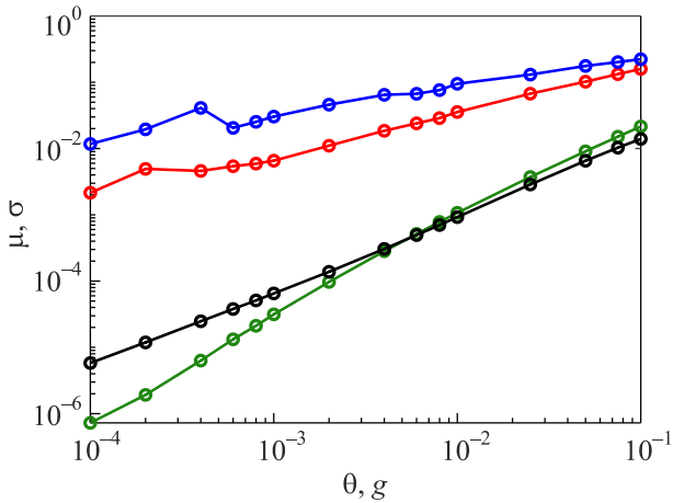
Fig. 11. (Color online) The average value ( \mu ) and standard deviation ( \sigma ) of the Lyapunov observable for the SRN and LRN cases, with both axes in \log_{10} scale. The red and blue lines represent the mean ( \mu ) and standard deviation ( \sigma ) of SRN with g = 1 and varying \theta ( 10^{-4} to 10^{-1} ). The green and black lines represent the mean ( \mu ) and standard deviation ( \sigma ) of LRN with \theta = 0.33\pi and varying g ( 10^{-4} to 10^{-1} ). The system size is N = 50 , and the evolution time is 10^9 . Similar to Fig. 4, the averages and standard deviations are calculated using 10^9 points.
