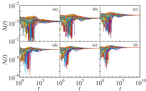
Fig. 13. (Color online) The time evolution of the largest Lyapunov exponent \Lambda(t) up to 10^{10} for different values of g for the LRN case ( \theta = 0.33\pi ) within the unitary circuits map. Panels (a) through (f) correspond to g = 0.001, 0.002, 0.004, 0.006, 0.008, 0.01 , respectively. Each panel shows 100 trajectories resulting from 100 different initial conditions, displaying the \Lambda(t) values on a \log_{10} scale. The system consists of N = 50 unit cells.
