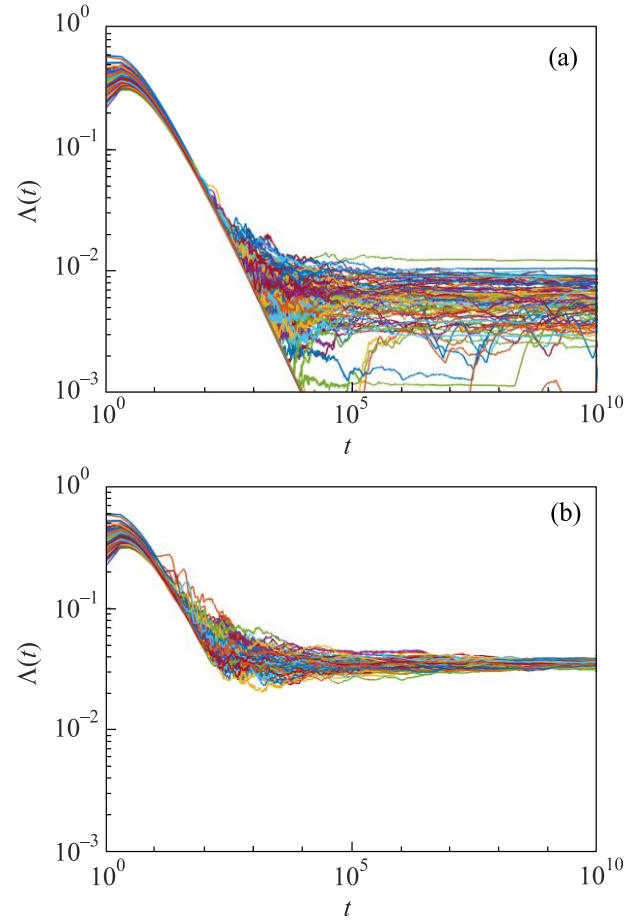
Fig. 6. (Color online) Same as Fig. 5 for the SRN case with g = 1 and \theta = 0.001 (a) and 0.01 (b).
