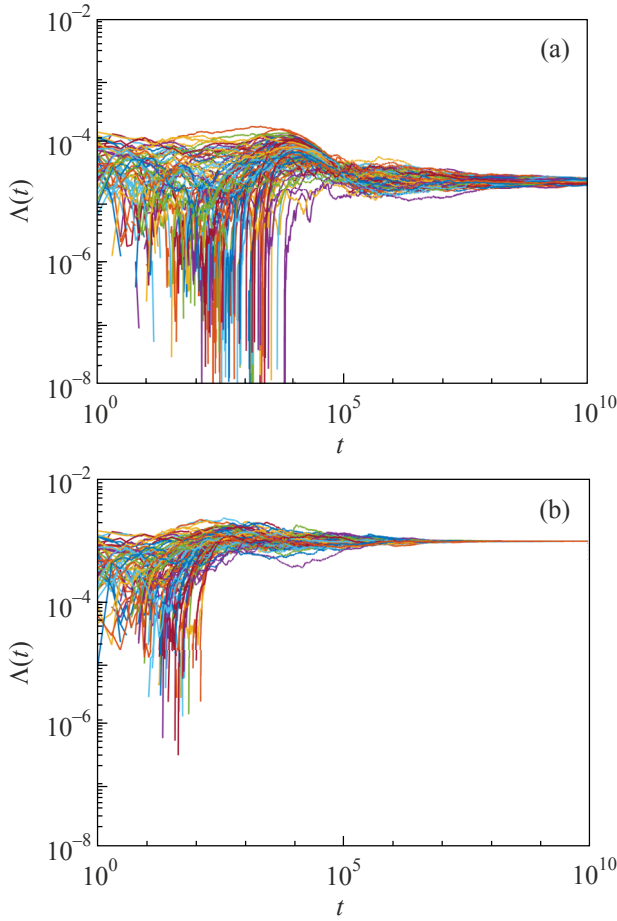
Fig. 5. (Color online) Time evolution of the largest Lyapunov exponent \Lambda(t) on a \log_{10} scale for up to 10^{10} iterations for g = 0.001 (a) and 0.01 (b) in the LRN case for \theta = 0.33\pi . Each panel shows 100 trajectories obtained from randomly chosen initial conditions. The system consists of N = 50 unit cells.
