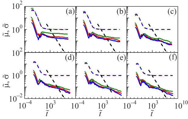
Fig. 10. (Color online) Same as Fig. 9 for the SRN case with g = 1 . Panels (a)–(f) correspond to \theta = 0.001, 0.002, 0.004, 0.006, 0.008, 0.01 , respectively.
