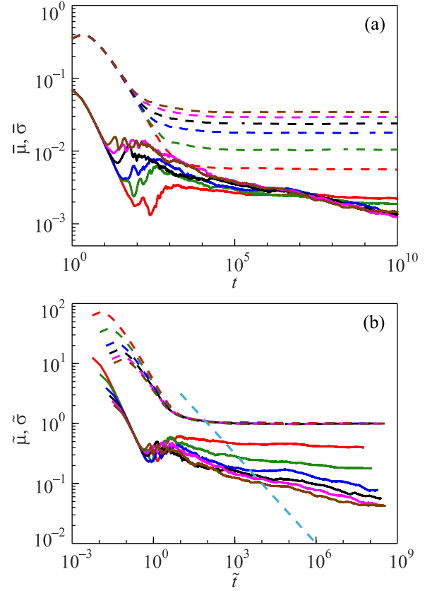
Fig. 8. (Color online) Same as Fig. 7 for the SRN case with g = 1 for different values of \theta . The colors red, green, blue, black, magenta, and brown correspond to \theta = 0.001, 0.002, 0.004, 0.006, 0.008, 0.01 , respectively.
