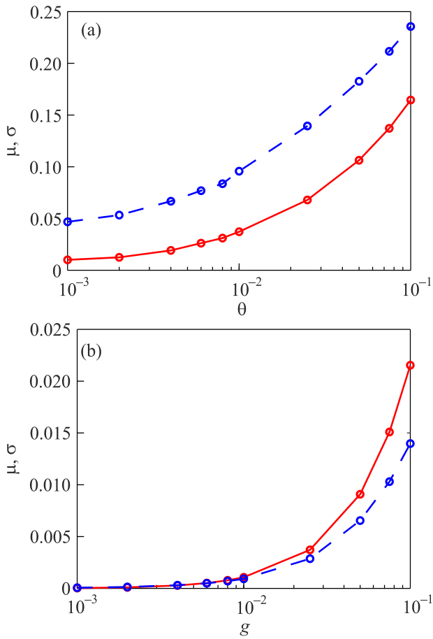
Fig. 4. (Color online) Average value, \mu , and standard deviation, \sigma , of the Lyapunov observable for the SRN and LRN cases, with both panels using a \log_{10} scale on the x axis. Panel (a) represents the SRN case with g = 1 and varying \theta , while panel (b) shows the LRN case with \theta = 0.33\pi and varying g . The red solid line represents the mean value ( \mu ), and the blue dashed line represents the standard deviation ( \sigma ). The circles correspond to the specific values of g or \theta used in the calculation. The unitary map Eq. (1) is iterated 10^9 times, yielding 10^9 values for r(t) that were all used to compute the mean and standard deviations. The system consists of N = 100 unit cells.
