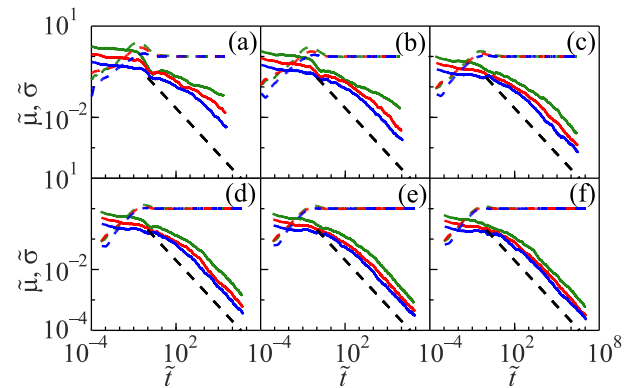
Fig. 9. (Color online) Average scaled mean ( \tilde{\mu} , dashed lines) and standard deviation ( \tilde{\sigma} , solid lines) of \Lambda calculated from 100 trajectories at each time step for the LRN case with \theta = 0.33\pi . Panels (a)–(f) correspond to g = 0.001, 0.002, 0.004, 0.006, 0.008, 0.01 , respectively. The black dashed line shows the expected temporal decay, \sigma \sim t^{-1/2} . Green, red, and blue curves indicate system sizes N = 50, 100, 200 , respectively. All data are plotted on a \log_{10} scale.
