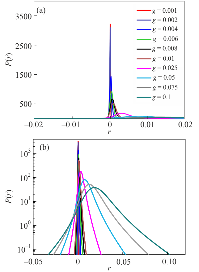
Fig. 3. (Color online) Same as Fig. 2 for the LRN case with \theta = 0.33\pi . The colors corresponding to the different values of g in (a) and (b) are shown in the legend of panel (a).
