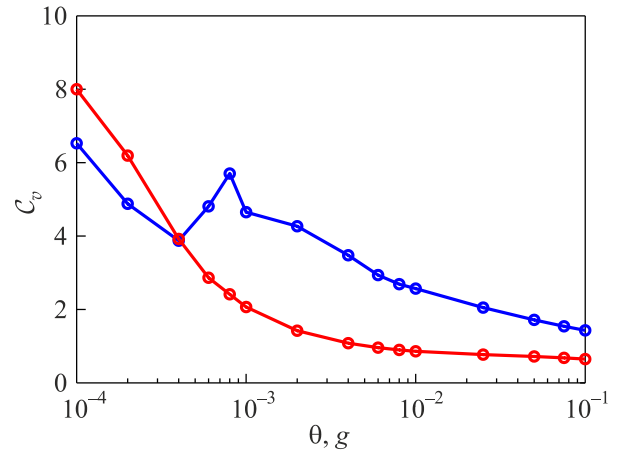
Fig. 12. (Color online) The coefficient of variation \mathcal{C}_v for the Lyapunov observable in the SRN and LRN cases, where \mathcal{C}_v = \sigma / \mu is the ratio of the standard deviation ( \sigma ) to the mean value ( \mu ). The blue line represents the SRN case with g = 1 and varying \theta ( 10^{-4} to 10^{-1} ), while the red line corresponds to the LRN case with \theta = 0.33\pi and varying g ( 10^{-4} to 10^{-1} ). The system size is N = 50 , and the evolution time is 10^9 .
