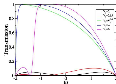
FIG. 6. (Color online) Transmission coefficient T vs frequency \omega_q for the three-site interaction, for different values of V_1 = V_{-1} . Other parameters are C = 1 , V_0 = 3 , and E_d = 0 . According to Eq. (25), perfect transmission starts to occur inside the spectrum for V_1 > 1.5 . There is an interval for coupling coefficient V_1 , when there is no perfect reflection inside the spectrum. For larger values of V_1 , both perfect transmission and perfect reflection move to the middle of the spectrum \omega_q = 0 .
