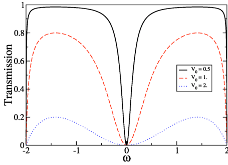
FIG. 2. (Color online) Transmission coefficient (8) calculated for the linear Fano-Anderson model (2) in the case E_d=0 , C=1 , and \lambda=0 , for several values of the coupling coefficient V_0 .
