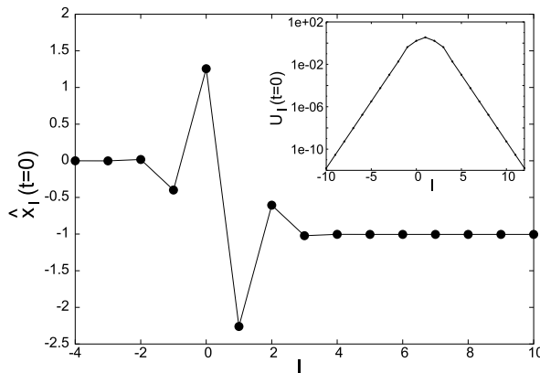
Fig. 6. An acoustic DB solution for the d = 1 case. Displacements X_l(t = 0) for \phi_2 = \phi_3 = \phi_4 = 1 and \Omega_b = 4.5 are plotted versus lattice site number l . At this initial time all velocities P_l(t = 0) = 0 . Inset: Staggered deformation u_l = (-1)^l(x_l - x_{l-1}) for the same solution on a logarithmic scale versus lattice site number l . This DB is linearly unstable. Data from [11].
